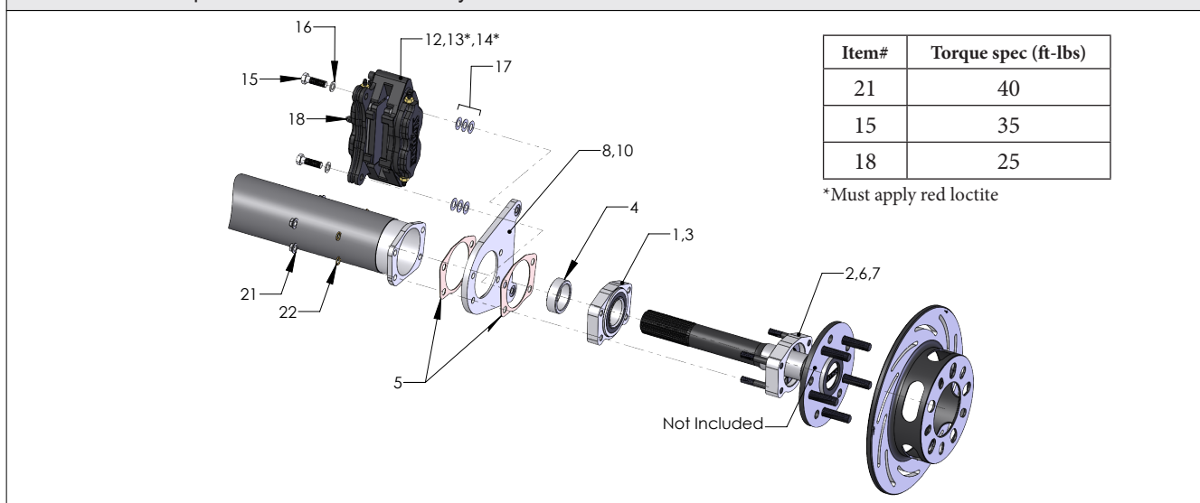
FIGURE # 1: Exploded B1714WC Assembly View
