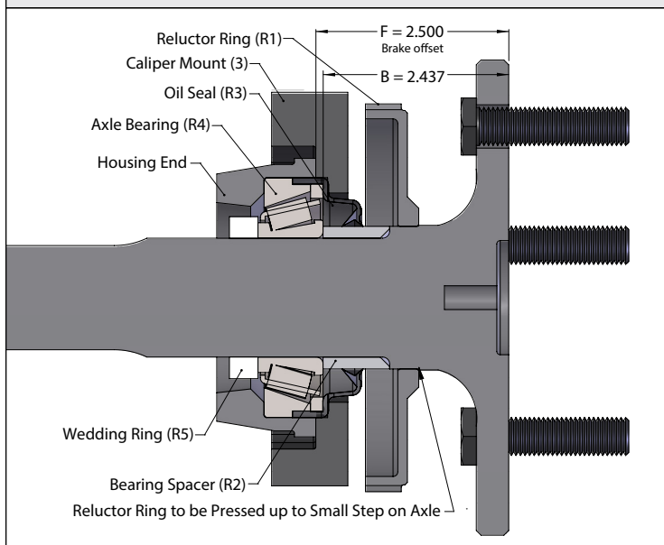
FIGURE # 1: Bearing Assembly (w/ optional abs)
