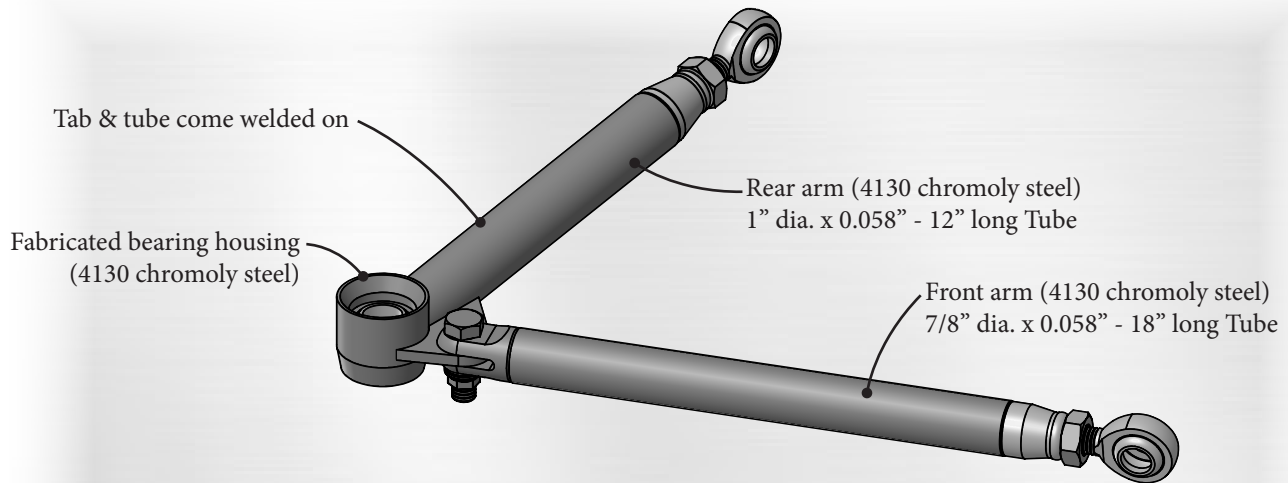
Fabricated Lower Control Arm (Passenger side shown)
