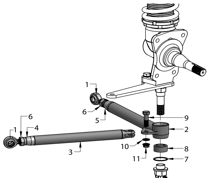
Exploded View (Driver side shown)
