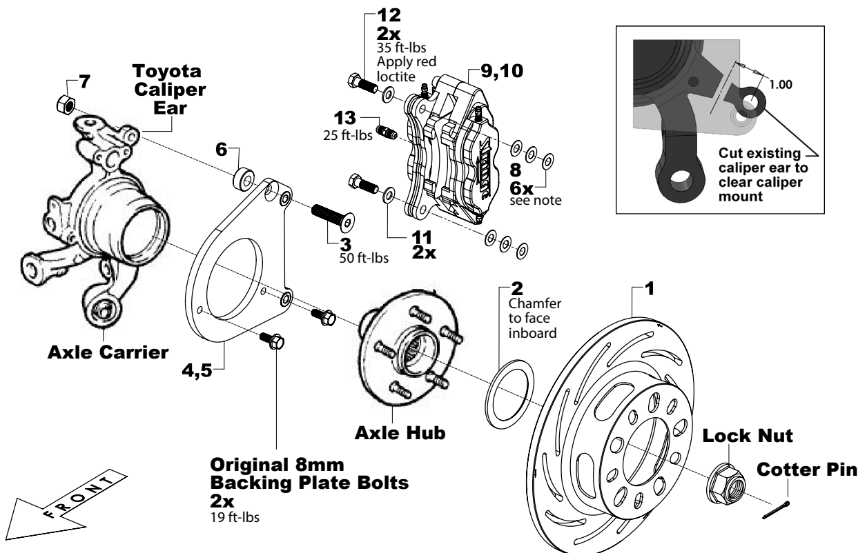
FIGURE # 2: Exploded B1720WC Assembly View
