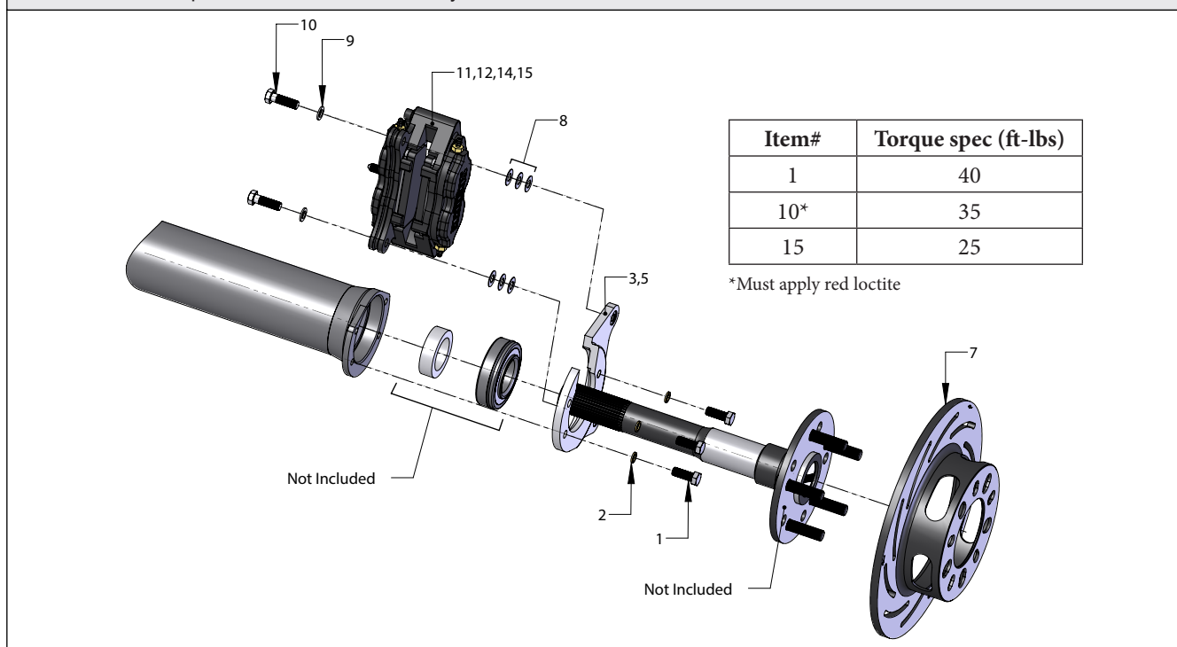
FIGURE # 1: Exploded B1750WC Assembly View
