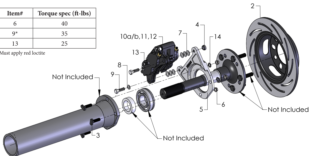
FIGURE # 1: Exploded B1708WC Assembly View
