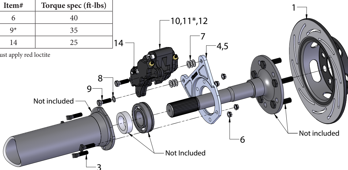
FIGURE # 1: Exploded B1706WC Assembly View
