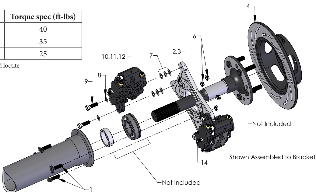
FIGURE # 1: Exploded B1700WCD Assembly View
