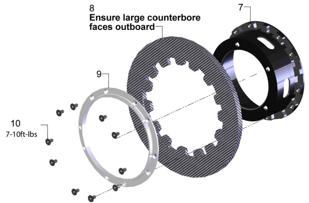
FIGURE # 2: Exploded B1200WC Assembly View
