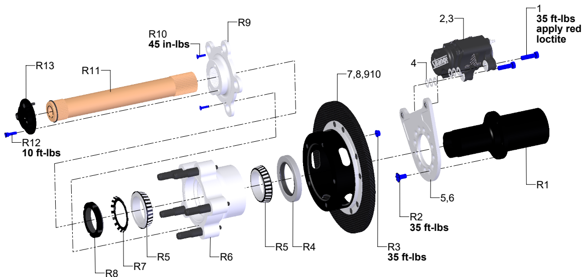
FIGURE # 1: Exploded B1200WC Assembly View
