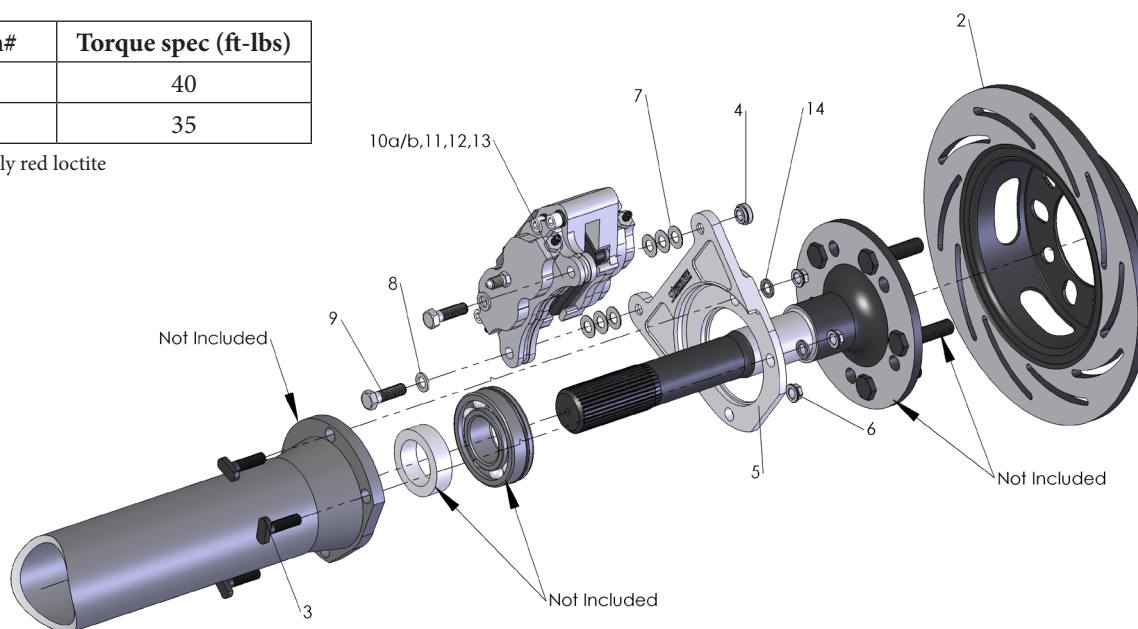
FIGURE # 1: Exploded B1708WC Assembly View
