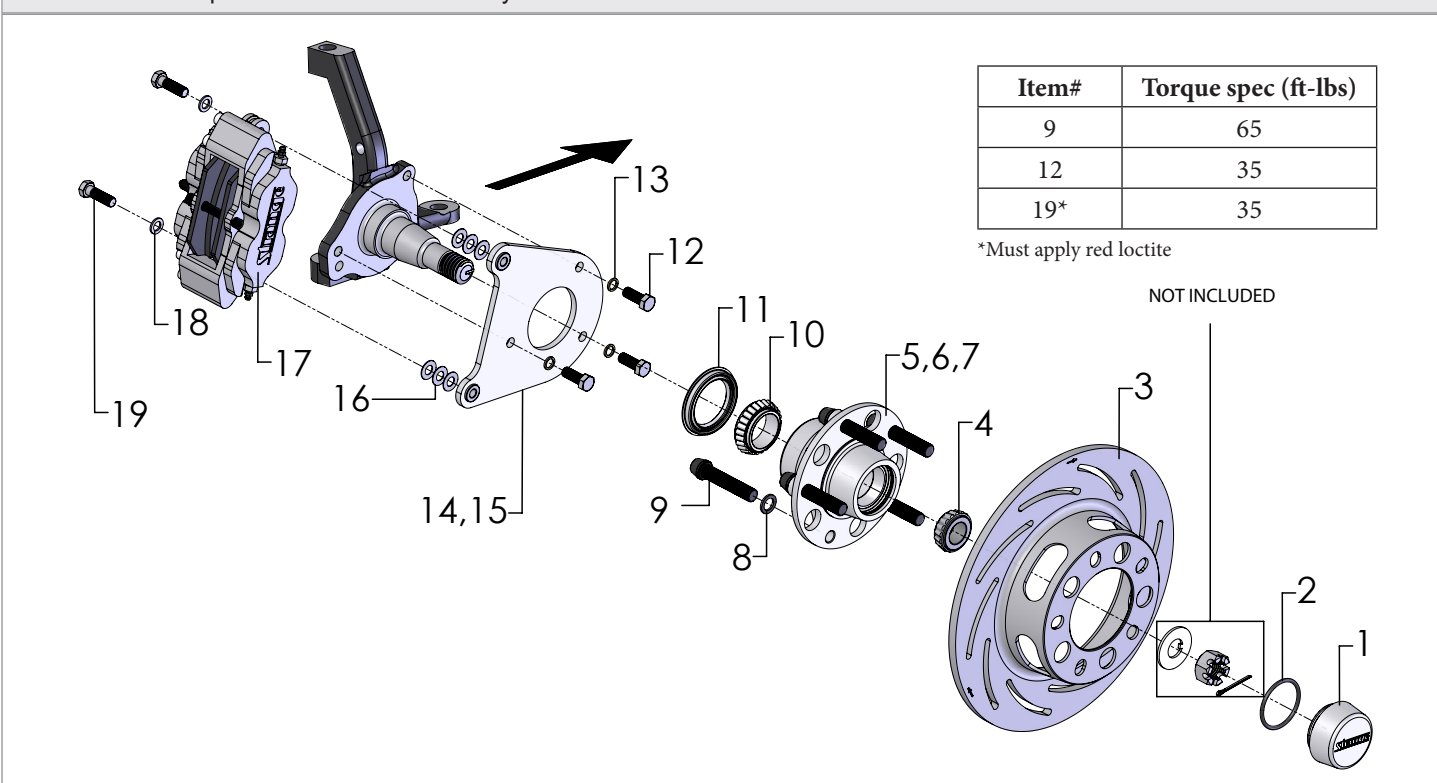
FIGURE # 2: Exploded B4140WC Assembly View
