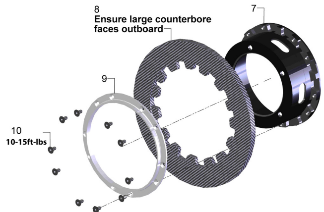
FIGURE # 1: Exploded B1200WC Assembly View
