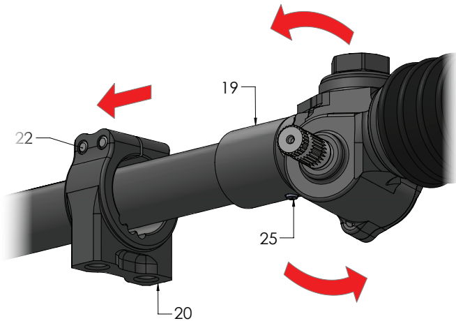
FIGURE# 1: DISASSEMBLY
