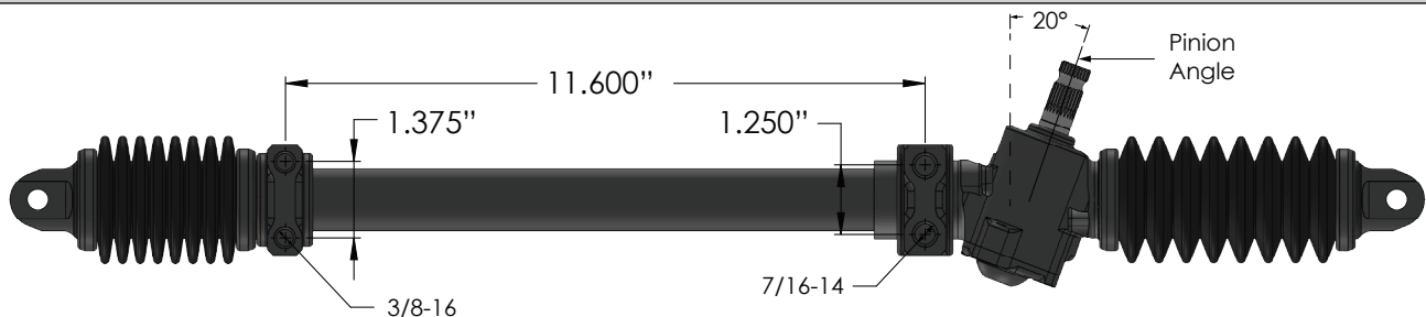
S3448RH Steering rack mounting dimensions
