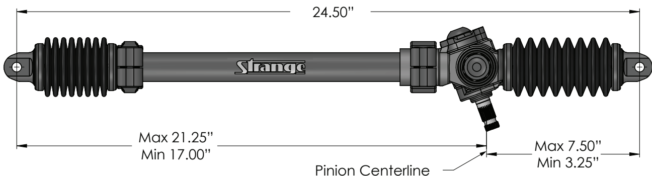
S3448RH Steering rack total travel
