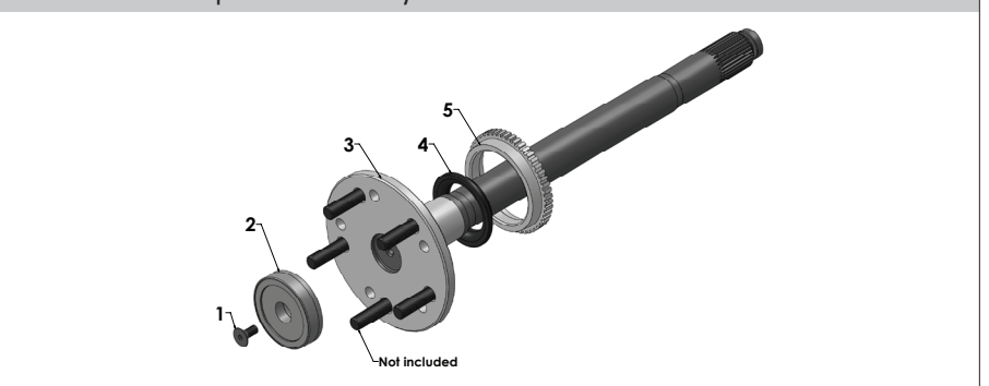
FIGURE # 4: Exploded assembly
