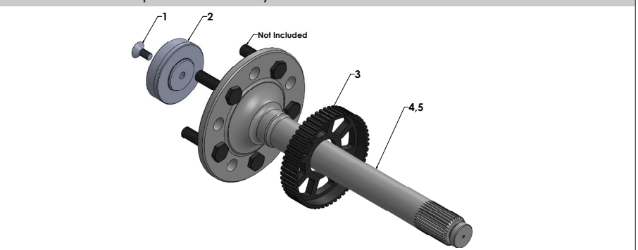
FIGURE # 2: Exploded assembly
