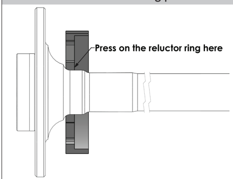
FIGURE # 1: Reluctor ring placement
