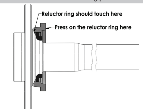
FIGURE # 3: Reluctor ring placement
