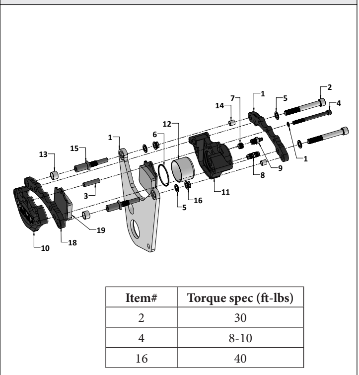
FIGURE # 2: Strange Evolution 1 Caliper Components
