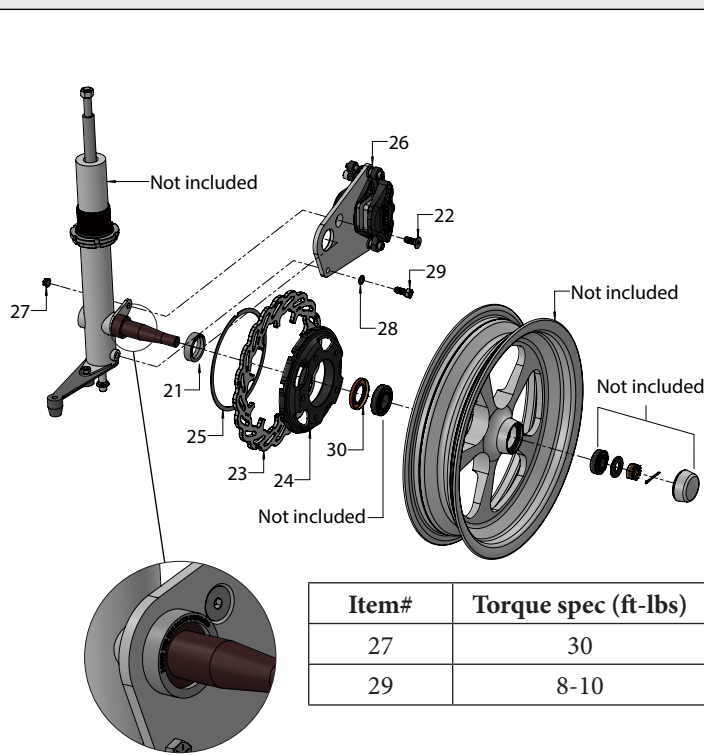
FIGURE # 1: Exploded B4500WCE Assembly View
