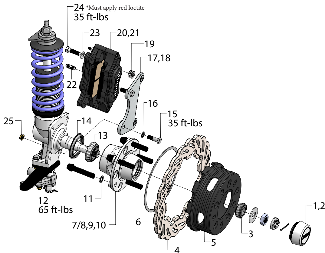
FIGURE # 2: B4153WCE/B4154WCE Exploded view
