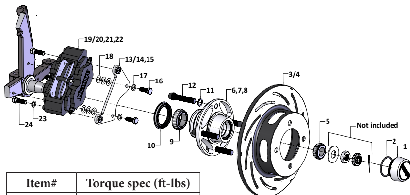
FIGURE # 2: Exploded B4147WC Assembly View (Passenger side)
