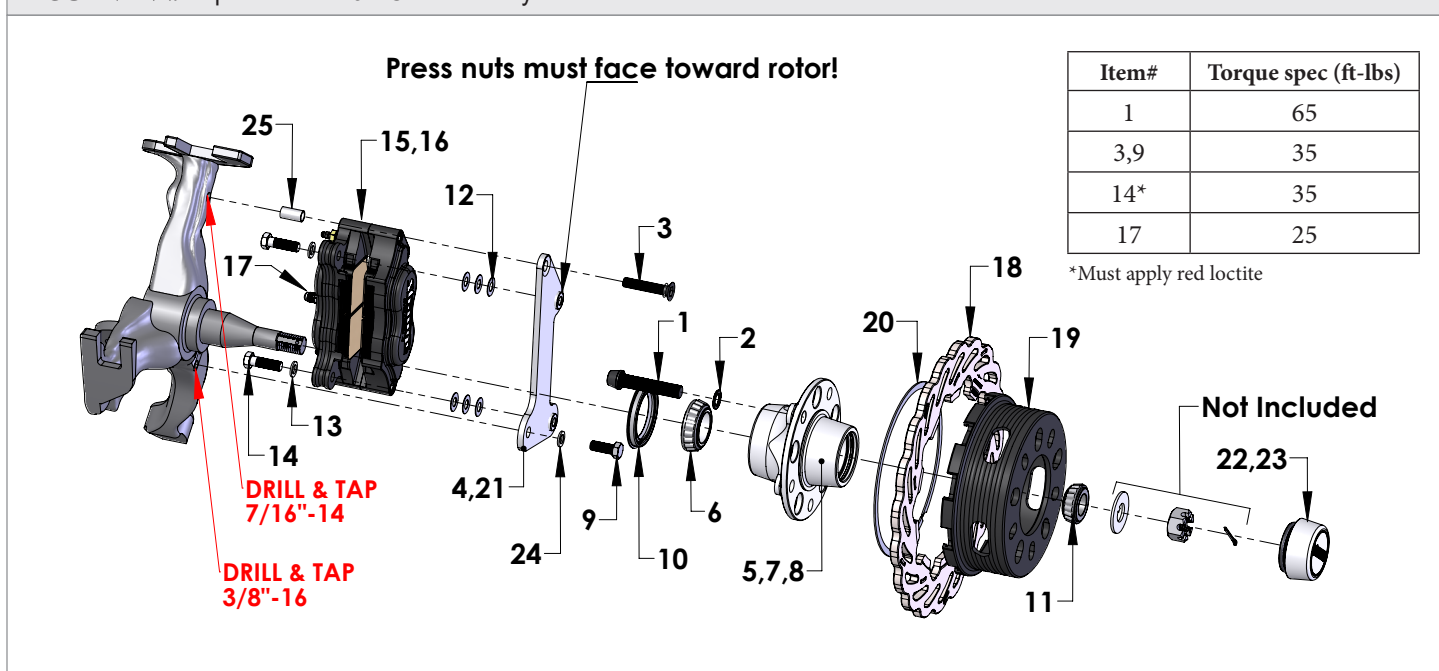
FIGURE # 2: Exploded B4116WCE Assembly View
