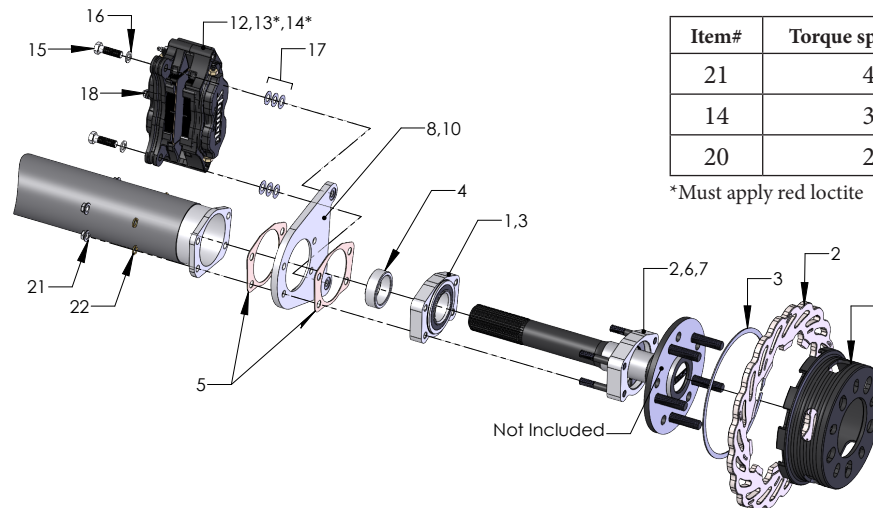
FIGURE # 1: Exploded B1714WC Assembly View
