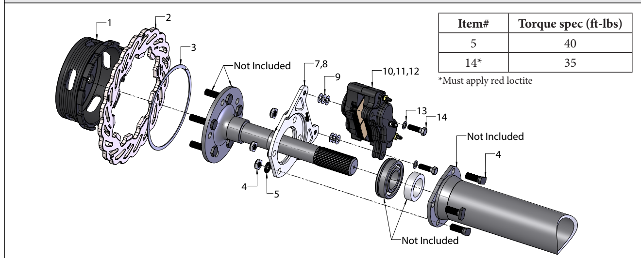
FIGURE # 1: Exploded B1707WCE Assembly View
