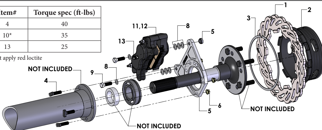
FIGURE # 1: Exploded B1700WCE Assembly View
