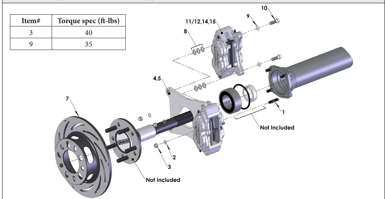
FIGURE # 1: Exploded B1711WCD Assembly View
