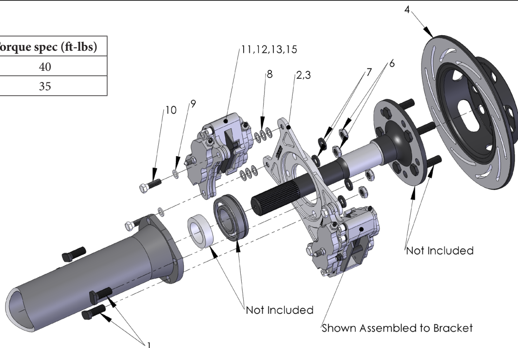
FIGURE # 1: Exploded B1708WCD Assembly View
